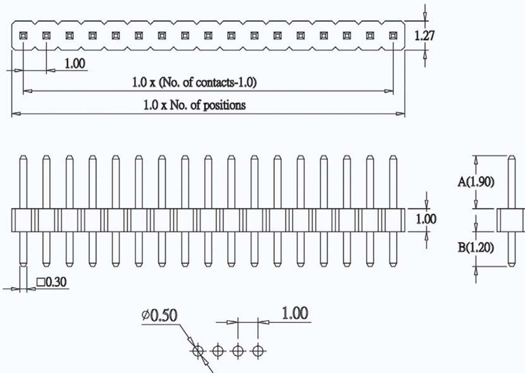
Recommended PCB Layout (PCB TOLERANCE ±0.05)
